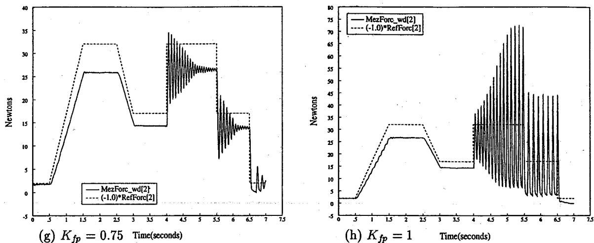
Fig. 8. continued. Experimental data of proportional gain explicit force control with feedforward. The proportional gain varies from -0.75 to 1 .
