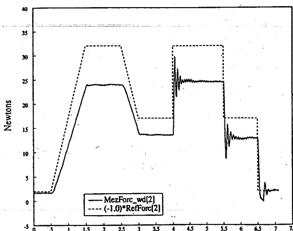
(e) K_{fp} = 0.25 Time(seconds)
