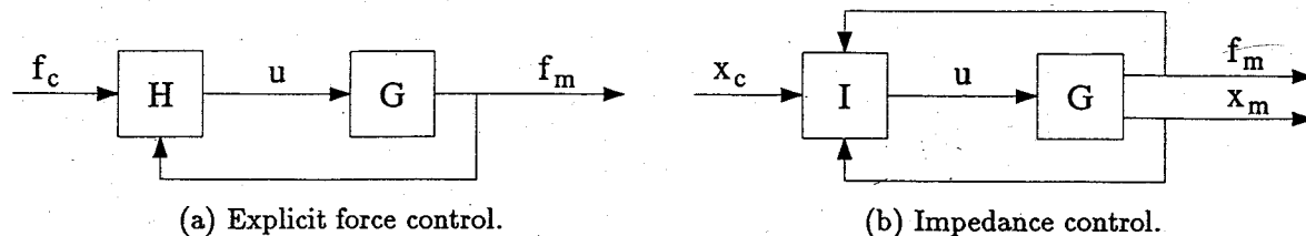
Fig. 1. Block diagrams of the two main types of force regulation.
