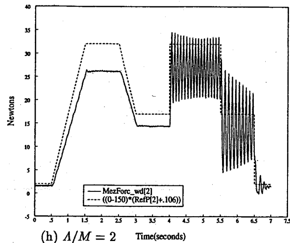
Fig. 9. continued. Experimental data of impedance control without dynamics compensation. The mass ratio "gain" varies from 0.25 to 2.0.
