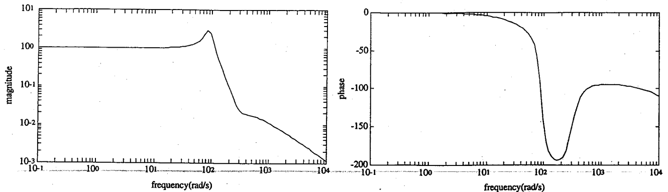
Fig. 6. Bode plots for the fourth-order system under proportional gain explicit force control. The resonance peak occurs near the natural frequency of the environment. The gain margin is 1.2 at \omega = 118 rad/s, which corresponds to the root locus crossing to the right half-plane in Figure 5.
