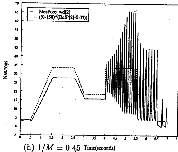
Fig. 10. continued. Experimental data of impedance control with dynamics compensation. The commanded inverse mass varies from 0.1 to 0.45. This is approximately the same as 0.5 \leq \Lambda/M \leq 2.25 and -0.5 \leq K_{fp} \leq 1.25 .
