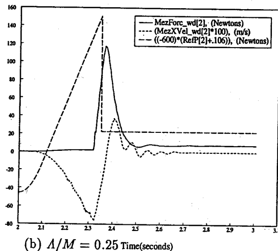
Fig. 11. Experimental data comparing the best response for impacts controlled by proportional gain explicit force control with feedforward force, and those controlled by impedance control. The controllers have essentially equivalent response and are well suited for ensuring impact stability with the proper selection of control parameters.
