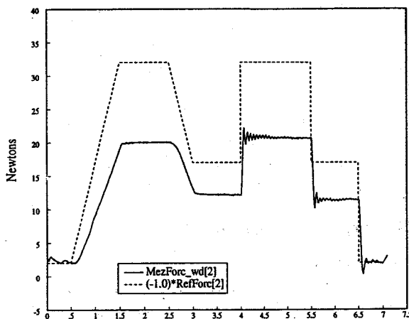
(c) K_{fp} = -0.25 Time(seconds)
