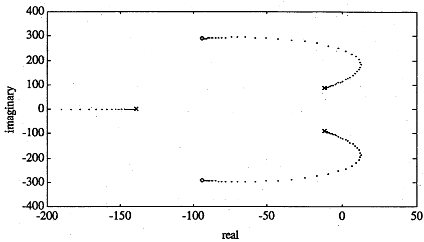
Fig. 4. Root locus for the fourth-order model under proportional gain explicit force control ( K_{fp} \geq 0 ).
