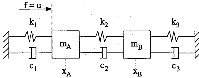
Fig. 3. General fourth-order model of the arm, sensor, and environment system.
