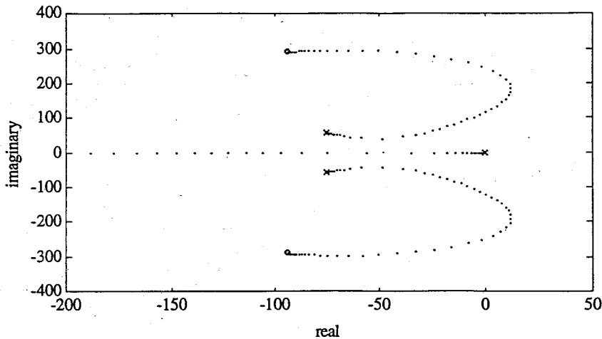
Fig. 7. Root locus for the fourth-order model for -1 \leq K_{fp} < \infty or 0 \leq K'_{fp} < \infty .
