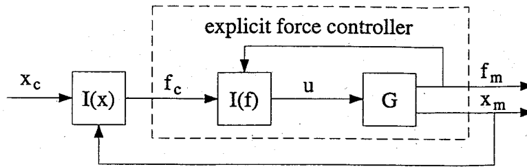
Fig. 2. Impedance control block diagram redrawn to show the inner explicit force controller.
