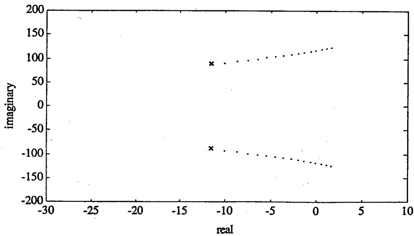
Fig. 5. Enlargement of the root locus in figure 4 with K_{fp} values of 0 to 1.5 in steps of 0.1.
