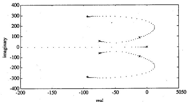
Fig. 12. Root locus for the fourth-order model for -1 \leq H < \infty or 0 \leq H' < \infty . The poles shown in the middle of the locus are for H = 0 and correspond to the environmental pole locations in Figure 3.
