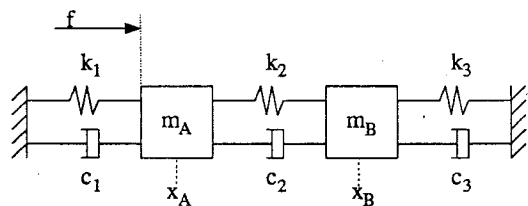
Fig. 2. General fourth-order model of the arm, sensor, and environment system.
