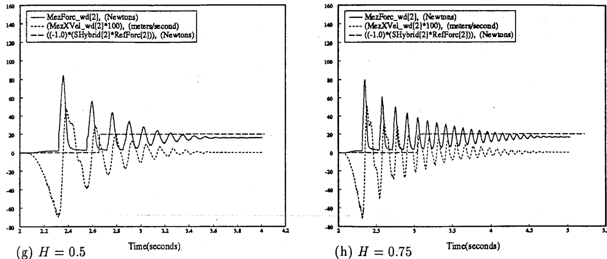
Fig. 14. A–F, Experimental data of proportional gain explicit force control with feedforward during impact. The proportional gain varies from -1 to 0.75 . G–H, Experimental data of proportional gain explicit force control with feedforward during impact. The proportional gain varies from -1 to 0.75 .
