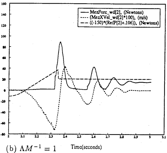
Fig. 16. Experimental data of impact control with transition to integral gain force control. The impact control phase lasts for 0.15s after the beginning of the impact. This is followed by a period of transition from impact control to integral gain force control that lasts 0.15 s. Beyond 0.3 s after impact, integral gain force control is used.
