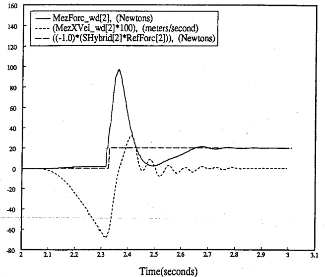
Fig. 16. Experimental data of impact control with transition to integral gain force control. The impact control phase lasts for 0.15s after the beginning of the impact. This is followed by a period of transition from impact control to integral gain force control that lasts 0.15 s. Beyond 0.3 s after impact, integral gain force control is used.
