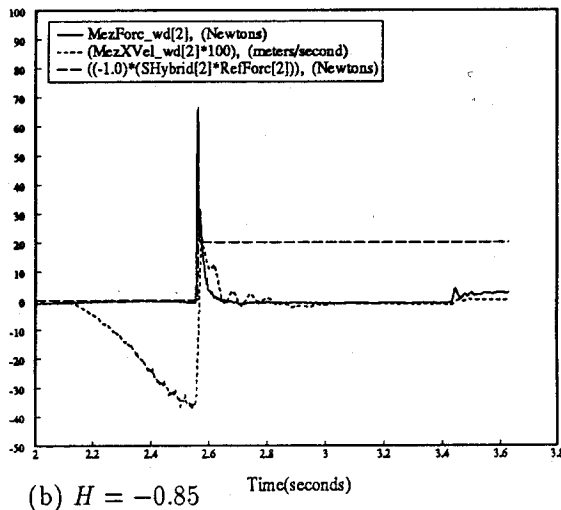
Fig. 17. Impact control on the steel pedestal in the z direction: comparison of H = 0 (open loop) and H = -0.85 .
