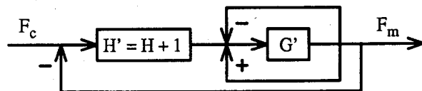
Fig. 9. Block diagram of a force-based explicit force controller with proportional gain and extra feedback for reaction force compensation. The plant G has been expanded into its components, and the sensor dynamics have been ignored.
