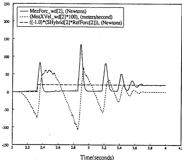
Fig. 13. Experimental data from an impact with integral force control. The integral gain was K_{fi} = 7.5 .
