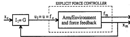
Fig. 7. Impedance control block diagram redrawn to show the inner explicit force controller.
