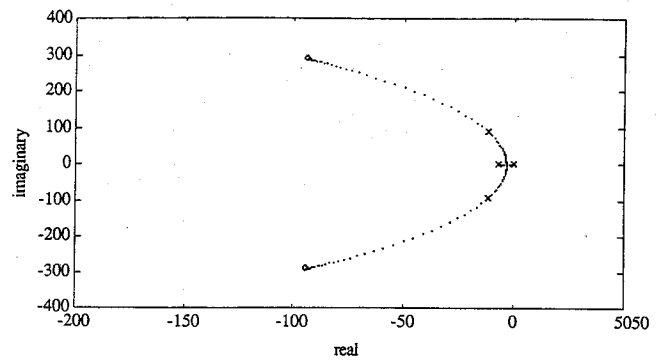
Fig. 11. Root locus for the second-order model for H' = H + 1 . The double root occurs for H' \approx 1.5 \times 10^{-3} . The poles shown in the middle of the locus are for H = 0 and correspond to the environmental pole locations in Figure 3.
