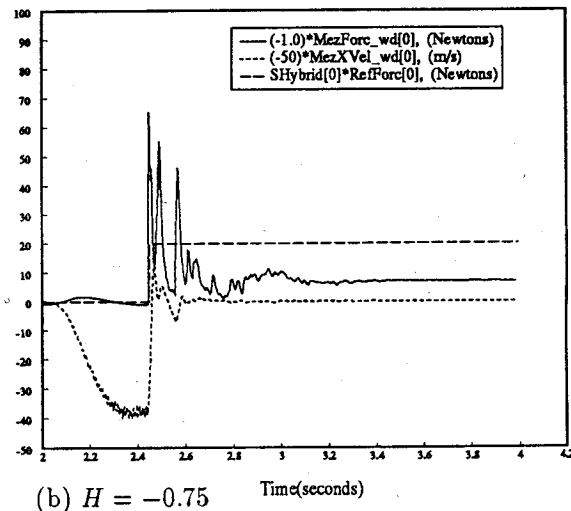
Fig. 18. Impact control on the steel pedestal in the x direction with H = 0.75 and -0.75 .
