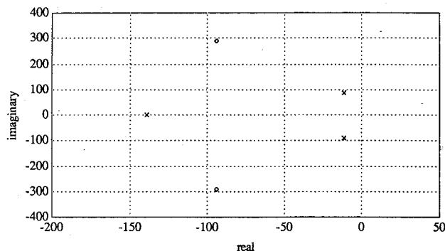
Fig. 3. The pole and zero locations for the fourth-order model using the experimentally extracted parameters. Not shown is the leftmost pole, which is at -28,000 on the real axis.
