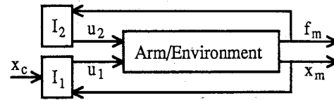
Fig. 6. Impedance control block diagram with the controller divided into its position part, I_1 , and its force part, I_2 .
