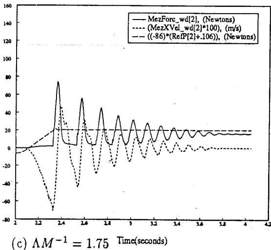
Fig. 15. Experimental data of impedance control during impacts for the stated mass ratios.
