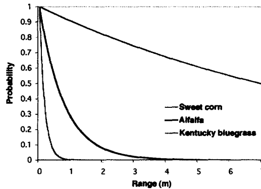
Fig. 2. Probability g(r) that a range measurement will reach an obstacle as a function of range, r , for selected crop data from Table 1
