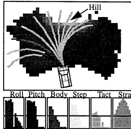
Figure 8: Onboard Obstacle Detection
