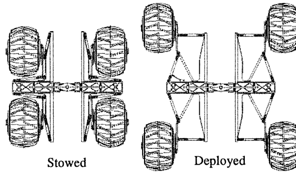
Figure 3: Transforming Chassis
