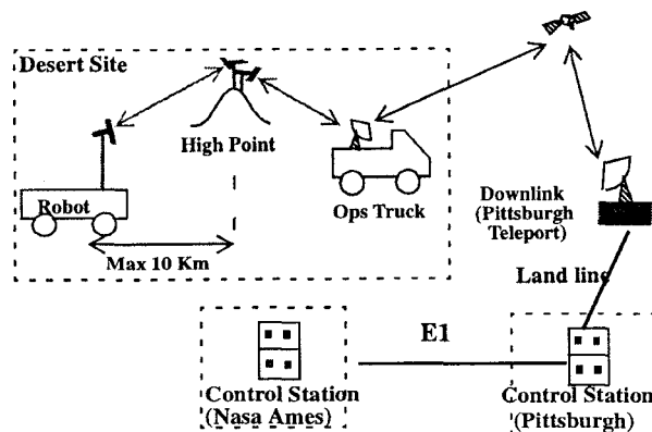
Figure 5: Communication Overview
