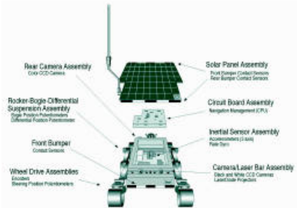
Figure 6 The Rover Assembly
