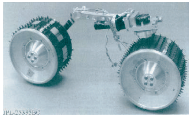
Figure 7 Reflective wheel (left) for WAE instrument
